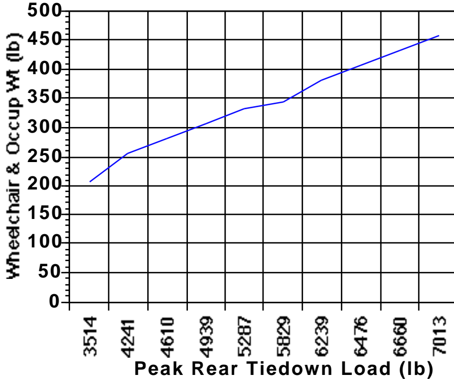
Figure 13 Rear Tiedown Loads for Varying Combined Wheelchair & Occupant Weight - 20g/30mph Frontal Crash Note: Lap belt anchored to wheelchair, shoulder belt anchored to vehicle.
