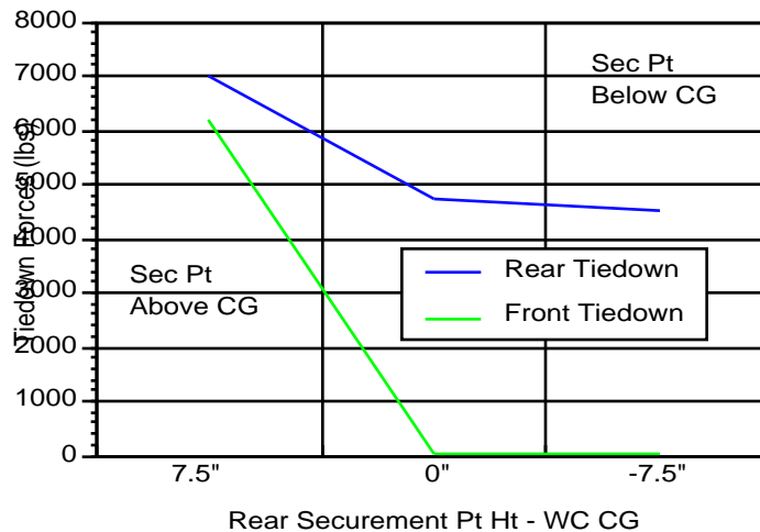
Figure 14 Rear Tiedown Load for Varying Securement Point Locations - 20g/30mph frontal crash
